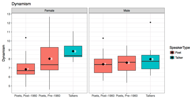
Figure 11. Dynamism, all
