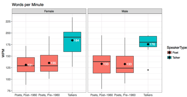
Figure 9. WPM, All
